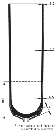
Dimension sketch:
